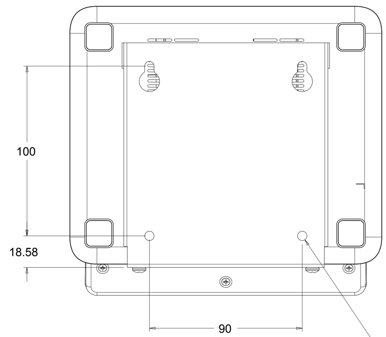
MOUNTING BRACKET USED FOR WALL
